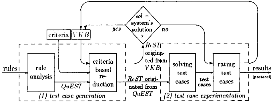
Fig. 1. The use of the VKB in the Validation Framework
