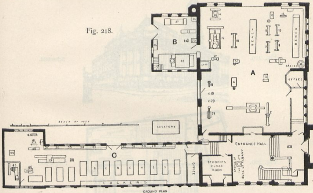
Walker Engineering Laboratories zu Liverpool 100 ).
