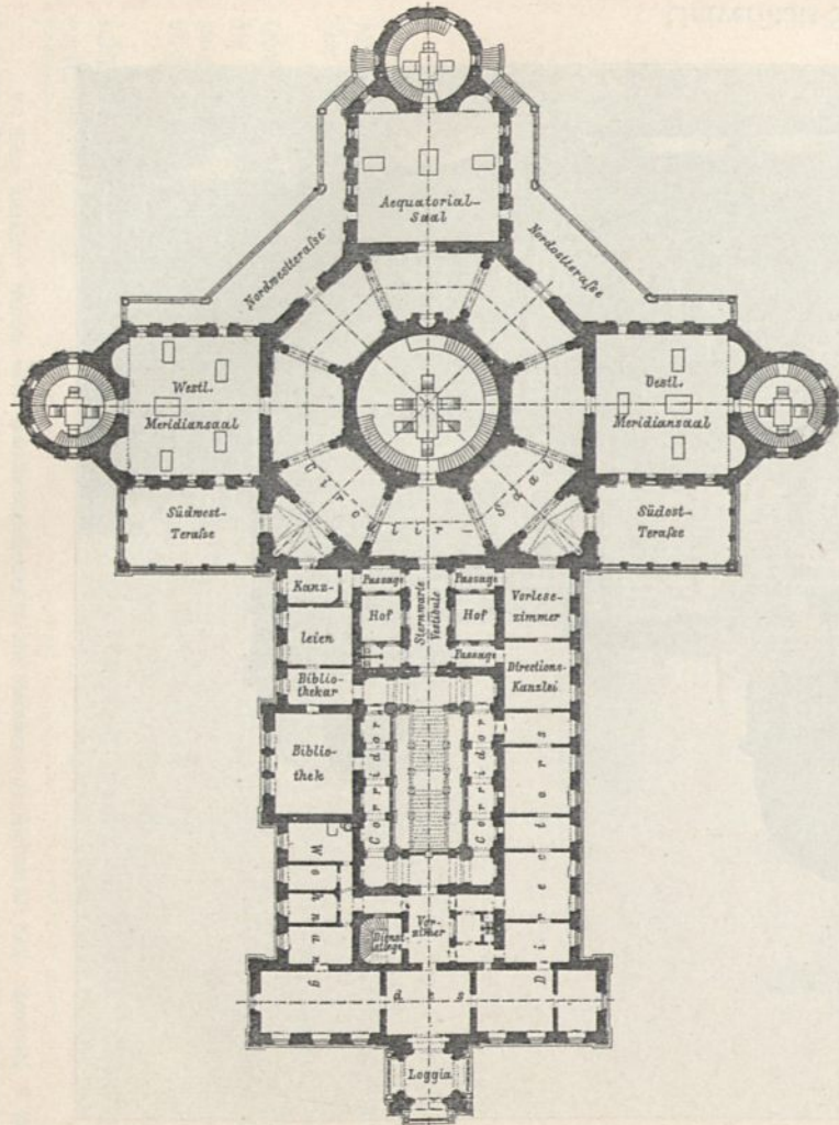
Erdgeschoss.
