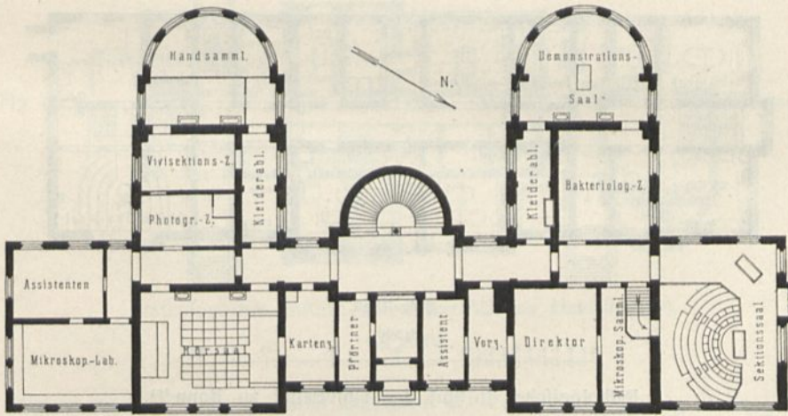
Erdgeschoss.
