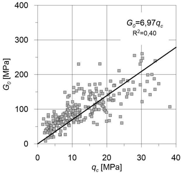
Figure 7: Correlation between shear modulus G_0 and cone resistance q_c for the entire data population.
