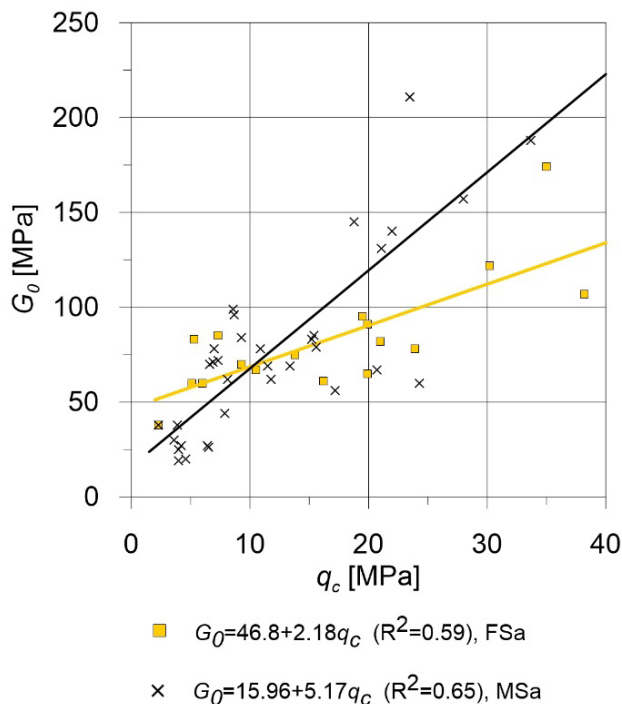
Figure 10: The correlation between modulus G_0 and cone resistance q_c for overconsolidated soils taking into account the type of soil.
