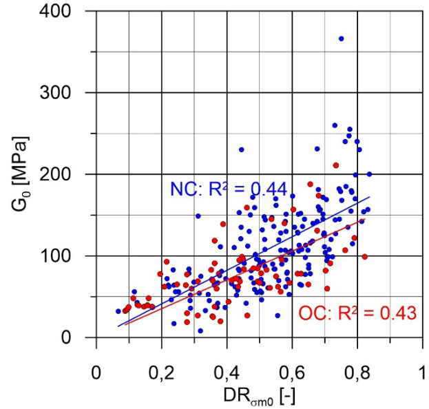
Figure 14: Correlation between G_o and D_r determined based on Eq. (14) taking into account \sigma'_{m0} .
