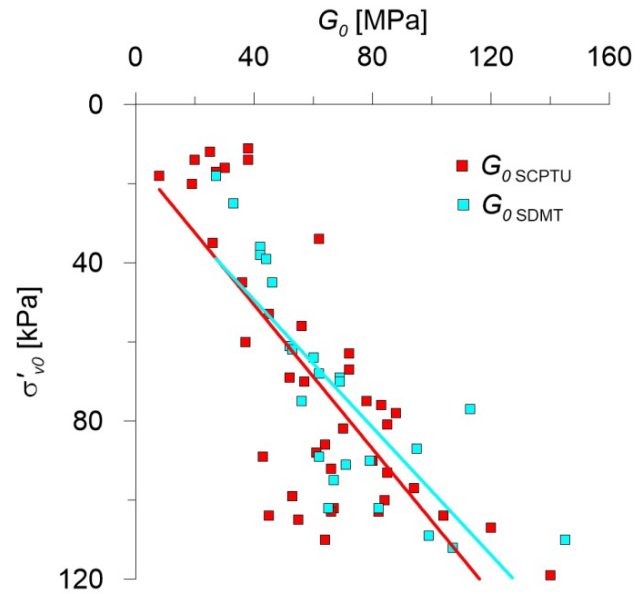
Figure 5: Trend of changes in shear modulus G_o with depth for SCPTU and SDMT performed in normally consolidated medium sands (data set from Derkacze and Gnojewo test sites).
