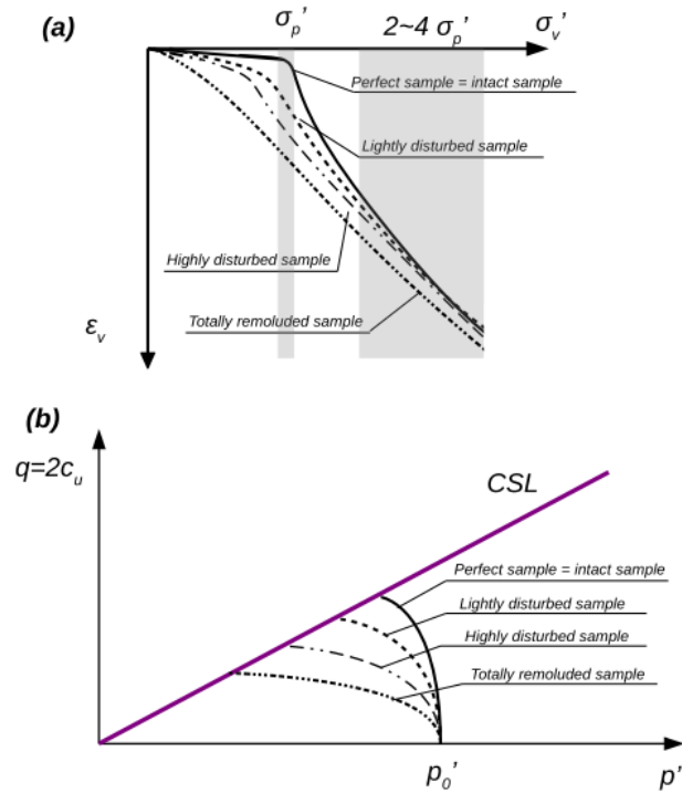
Figure 1: Schematic presentation of soft soil sample quality influence on (a) compressibility behavior and (b) undrained shear strength (Note: \sigma_v' = effective vertical stress; \epsilon_v = axial strain; \sigma_p' = preconsolidation pressure; q = deviatoric stress according to Cambridge notation; p' = effective mean stress according to Cambridge notation; p_0' = initial mean stress; CSL = critical state line).
