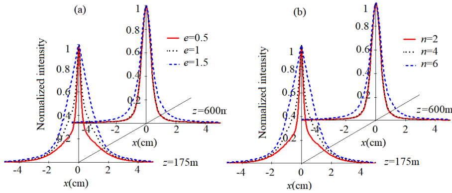
Fig. 5. Normalized intensity of EMHNUC beams at different positions with w_{0x} = 3 cm, w_{0y} = 2 cm, r_{xx} = 2 cm, and r_{yy} = 1 cm.
