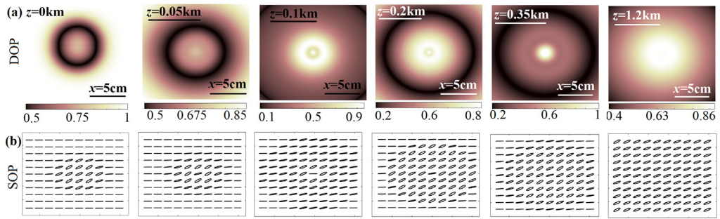
Fig. 3. Evolution of polarization characteristics of the EMHNUC beams in turbulence with (a) distribution of the DOP, and (b) distribution of the SOP. The parameter choices of the EMHNUC beams are the same as in Fig. 1(d).
