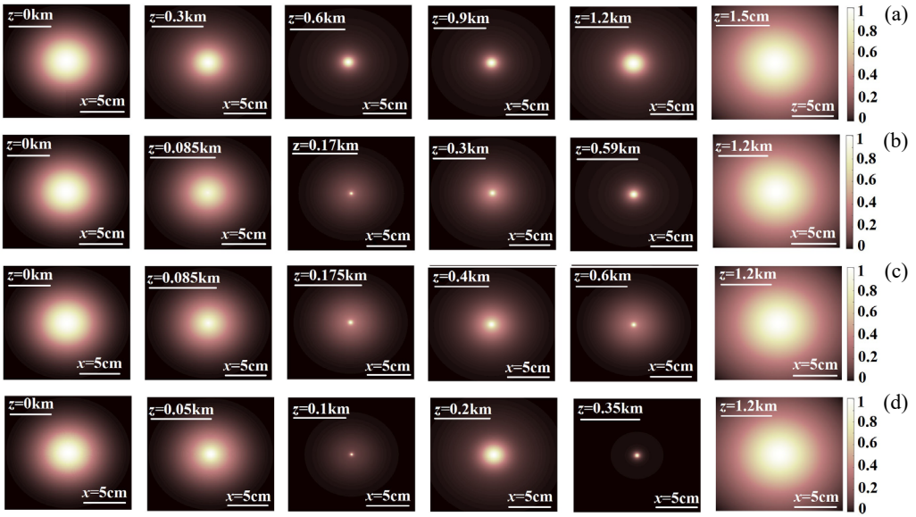
Fig. 1. Normalized intensity of the EMHNUC beams at different distances with different beam source parameters. (a) w_{0x} = w_{0y} = 3 cm, r_{xx} = r_{yy} = 2 cm; (b) w_{0x} = w_{0y} = 3 cm, r_{xx} = 2 cm, r_{yy} = 1 cm; (c) w_{0x} = 3 cm, w_{0y} = 2 cm, r_{xx} = 2 cm, r_{yy} = 1 cm; (d) w_{0x} = 3 cm, w_{0y} = 2 cm, r_{xx} = 2 cm, r_{yy} = 1 cm, n = 3 .
