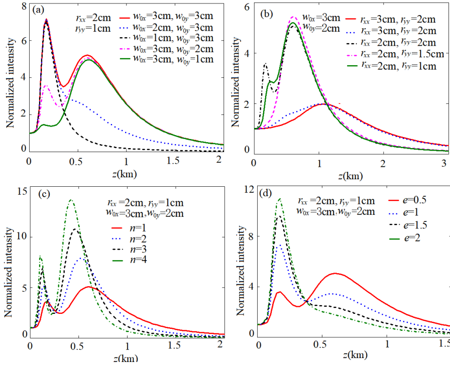
Fig. 4. On-axis distribution of normalized intensity of the EMHNUC beams for varying initial beam parameters and turbulence parameters. (a) For different w_{0x} and w_{0y} ; (b) for different r_{xx} and r_{yy} ; (c) for different n ; (d) for different e in a turbulent atmosphere.
