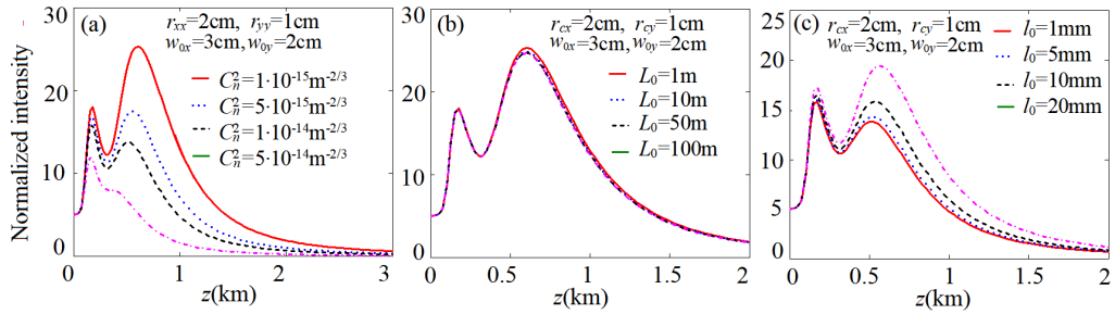
Fig. 6. Normalized intensity of EMHNUC beams at different turbulent parameters with w_{0x} = 3 cm, w_{0y} = 2 cm, r_{xx} = 2 cm, and r_{yy} = 1 cm.
