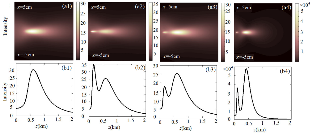
Fig. 2. Intensity distribution of the EMHNUC beam along the z -axis distance. The parameter selection from left to right is the same as the parameter selection in (a)-(d) in Fig. 1. (a) Intensity distribution of xoz plane. (b) On-axis intensity distribution along the z -axis.
