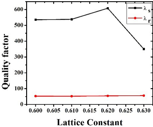
Fig. 6. Quality factor of sharp and broad peaks for different lattice constants.
