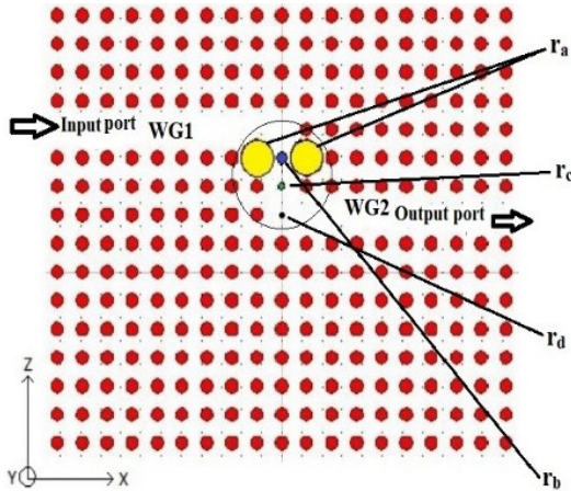
Fig. 3. Structure of the proposed sensor.
