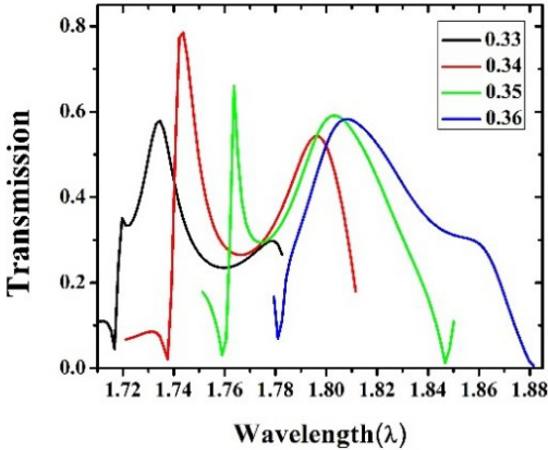
Fig. 7. Spectral response for different radius of scattering rod.
