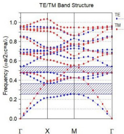
Fig. 2. Band diagram of the considered photonic crystal structure.
