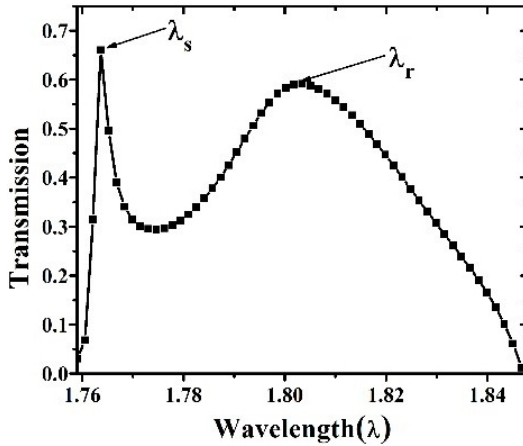
Fig. 4. Spectral response of the proposed sensor in the range of 1.76 to 1.845 \mu\text{m} .
