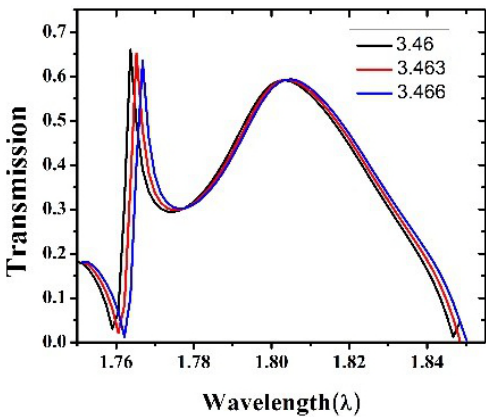
Fig. 8. Spectral response for different refractive-index of the rods.
