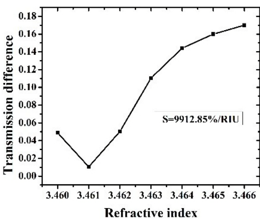
Fig. 13. Transmission difference vs. refractive-index.
