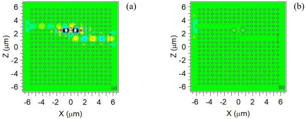
Fig. 9. Light propagation in the structure for 1.7637 \mu\text{m} ( \lambda_s ) when (a) RI = 3.46, and (b) RI = 3.466.
