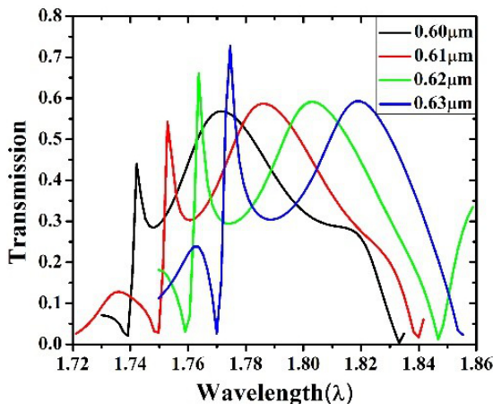
Fig. 5. Spectral response for different lattice constants.
