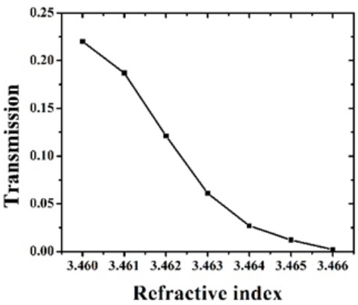
Fig. 11. Transmission vs. refractive-index for wavelength \lambda_s = 1.7637 \mu\text{m} .
