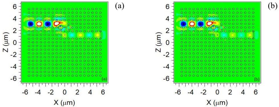
Fig. 10. Light propagation in the structure for 1.8033 \mu\text{m} ( \lambda_r ) when (a) RI = 3.46, and (b) RI = 3.466.
