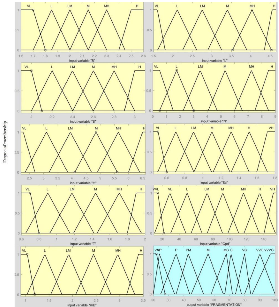
Fig. 6. Membership functions of inputs and output variables
