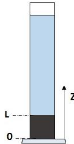
Fig. 2. Reference system used in the sediment in compression of a discontinuous sedimentation test.
