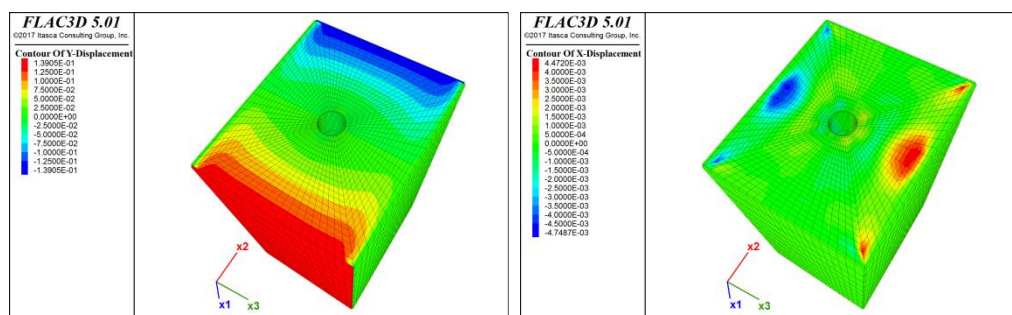
Fig. 7. Maps of displacements for horizontal soil compaction, directions: x_2 (left) and x_3 (right) – SN2, h = 2.0 m – values of cross-sectional deflection of manhole riser: -2.39 mm (axis x_2 ) and 2.03 mm (axis x_3 )
