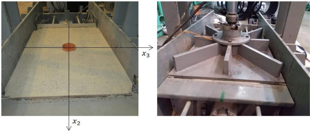
Fig. 3. Test stand box with a model of a flexible manhole riser in the soil (left) and a rigid steel plate which enables simulating vertical load on the soil (right)
