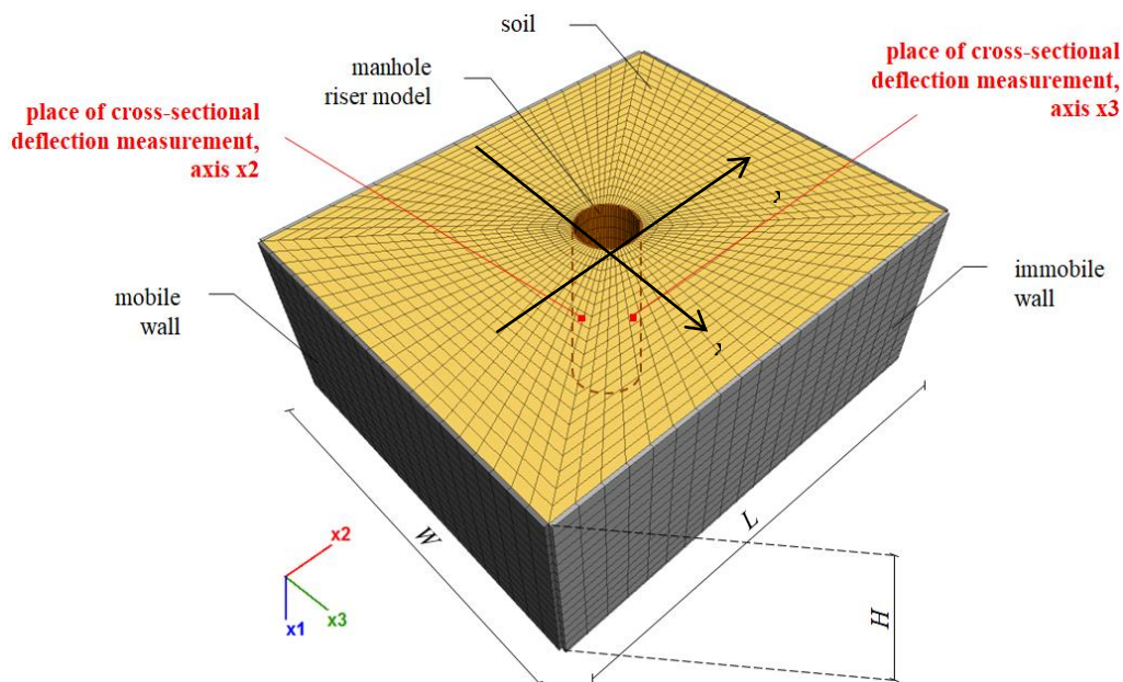
Fig. 2. Geometric model of the flexible manhole-soil interaction
