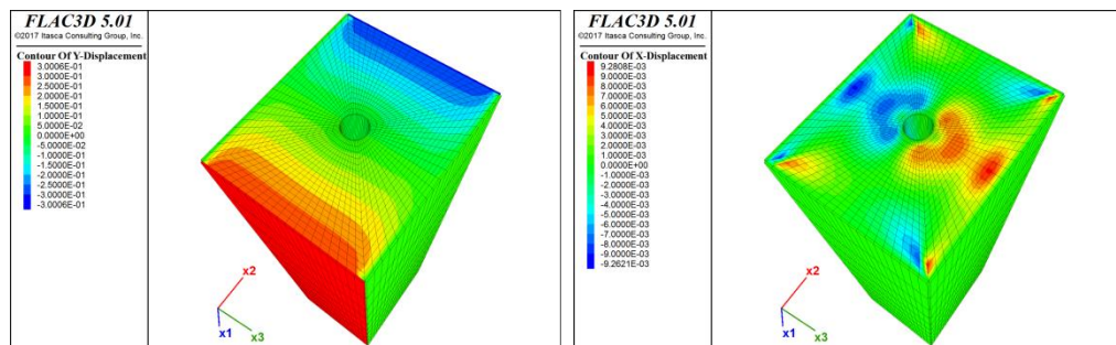
Fig. 6. Maps of displacements for horizontal soil compaction, directions: x_2 (left) and x_3 (right) – SN2, h = 4.0 m – values of cross-sectional deflection of manhole riser: -2.91 mm (axis x_2 ) and 2.67 mm (axis x_3 )
