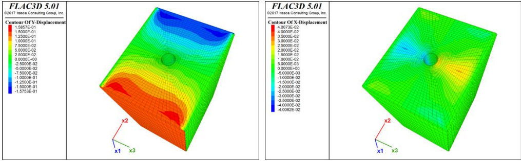
Fig. 9. Maps of displacements for horizontal soil compaction, directions: x_2 (left) and x_3 (right) – SN4, h = 2.0 m – values of cross-sectional deflection of manhole riser: -1.84 mm (axis x_2 ) and 1.57 mm (axis x_3 )
