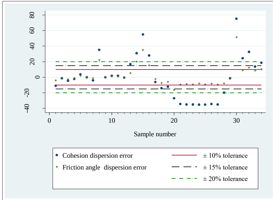
Fig. 5. Percentual error of cohesion and friction angle, when 20 \leq GSI' \leq 80 . Authors' own elaboration.
