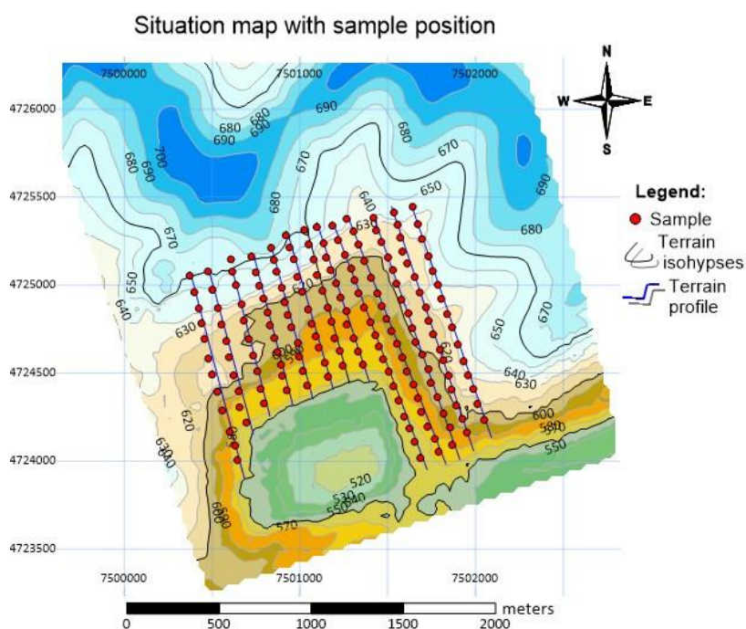
Fig. 1. Mine situation map with sample position M_1 – M_{127}
