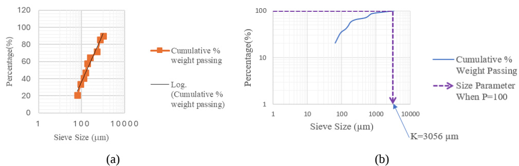
Fig. 10. Semi logarithm (a) and log-log (b) graph Product1 from Ball Mill for Test Ore (spodumene)
