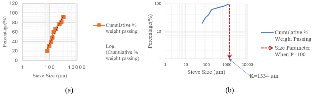
Fig. 14. Semi logarithm (a) and log-log (b) graph product from ball mill for reference sample (granite)
