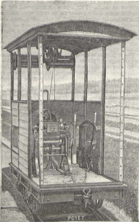
FIG. 1.—The locomotive, with dynamo-electric motor and driving-gear.
