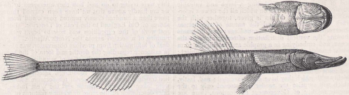
FIG. 2.— Ipnops Murrayi , Günth., 1600 to 1900 fathoms.
