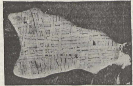
FIG. 2.—Section of Mazapil Meteoric Iron (natural size), showing Widmanstätten figures.
