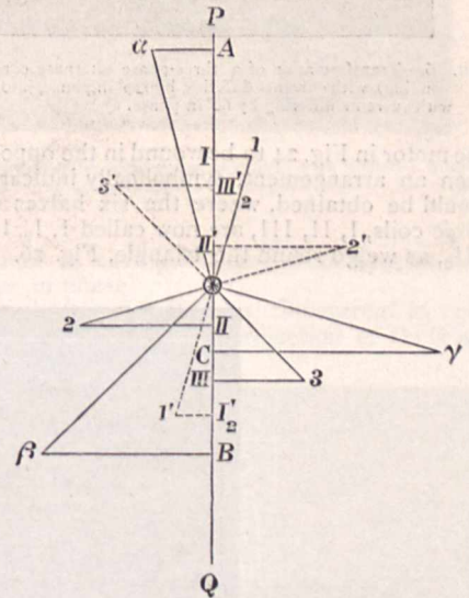
FIG. 25.—Projections of Oa, Ob, Oc give direction and relative magnitude of currents in the mains A, B, C of Figs. 20, 24, 27, 29, and 31, and of currents in coils I, II, III of Fig. 20. Projections of O1, O2, O3 completely represent currents in coils I, II, III of Fig. 24; and projections of O1, O2', O3' completely represent currents in coils I, II, III of Fig. 27. 4
