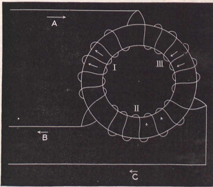
FIG. 24.—Three-phase alternate current motor (closed winding); currents differing by 120° in phase, and represented in direction and magnitude by the direction and length of the arrows.
