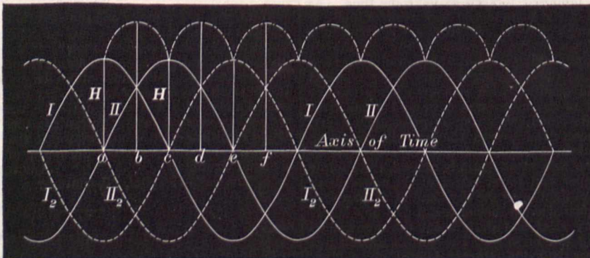
FIG. 17.—Two harmonic alternating currents of the same period and maximum amplitude, but differing by 90° in phase.
