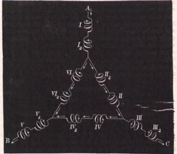
FIG. 30.—Transformation of an open wound combined with a closed wound six-phase alternate current motor into a twelve-phase motor with current differing by 30^\circ in phase.
