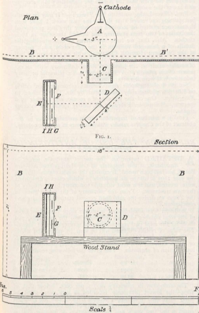
FIG. 2.—A, vacuum tube; BB', lead plate, 18 in. x 12 in. \frac{1}{8} in. thick; C, hole 2 in. diameter. Pipes 2 in. diameter x \frac{1}{2} in.; D, speculum-metal mirrors; E, zinc box, 4 in. x 4 in., 1 in. deep; F, aluminium window; G, objects; H, black cardboard; I, photographic plate.
