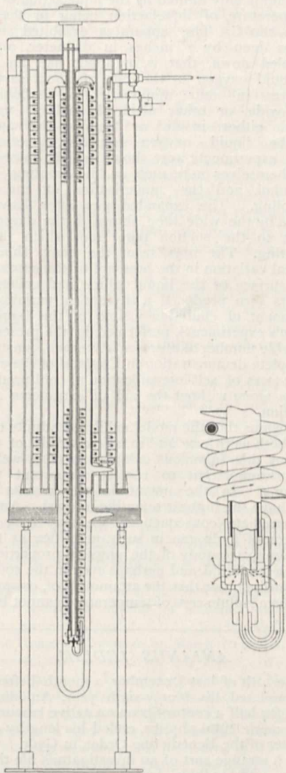
FIG. 1.—Sectional elevation.
