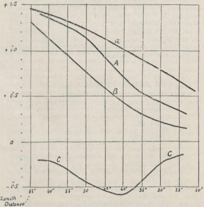
FIG. 2.— a , Flexure curve, 2(0''.80 \text{ sine zenith distance}) . A, R-D curve, south stars, reflex observation taken first. B, R-D curve, north stars, reflex observation taken first. C, R-D curve, south stars, direct observation taken first.
