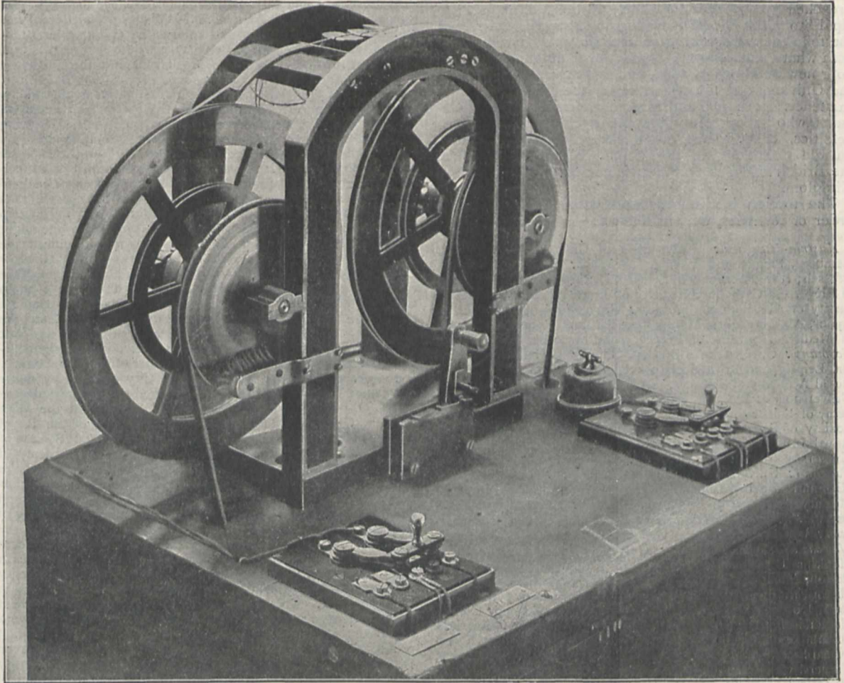
FIG. 2.—Steel Ribbon Telegraphone. (From the Electrician .)
