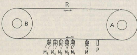
FIG. 3.—Distributing Telegraphone.
