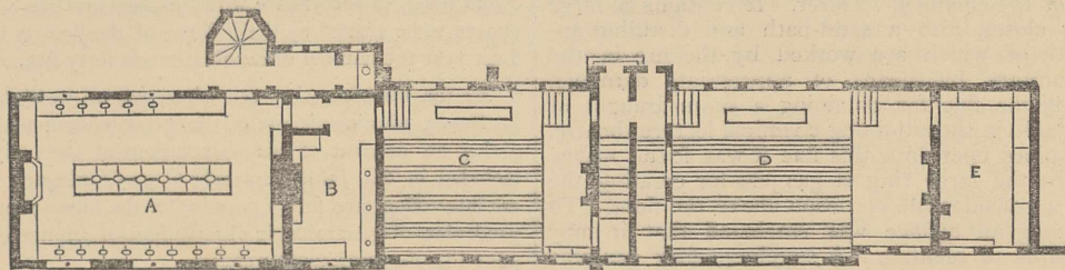
GROUND PLAN
