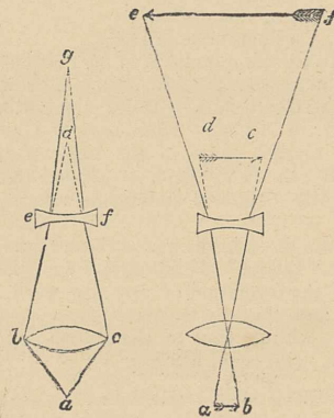
Fig. 1. b c , object glass; ef , Barlow lens; d g , foci of b c , with and without Barlow lens.
