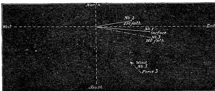
FIG. 2.—Rate (per hour) and Direction of Movement of Surface-Float, and of Current-Drag at different Depths; with Force and Direction of Wind in No. 3. (No Wind in Nos 1, 2.)
