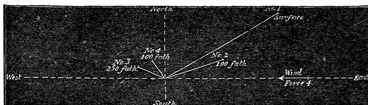
FIG. 1.—Rate (per hour) and Direction of Movement of Surface-Float, and of Current-Drag at different Depths; with Force and Direction of Wind.
