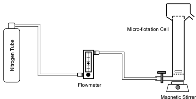
Fig. 4. Micro-flotation experimental setup
