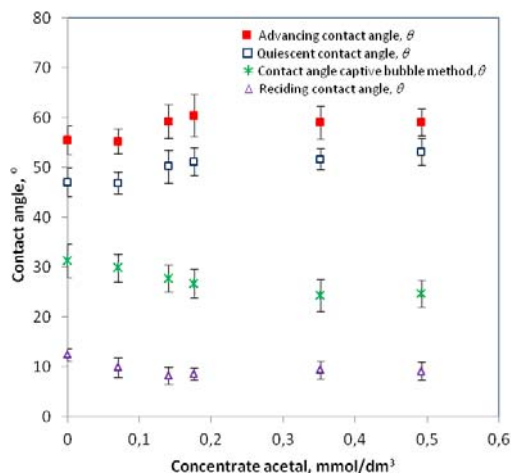
Fig. 6. Summary of the contact angle values of copper-bearing shales obtained using the sessile drop and captive bubble methods in function of acetal solution concentration
