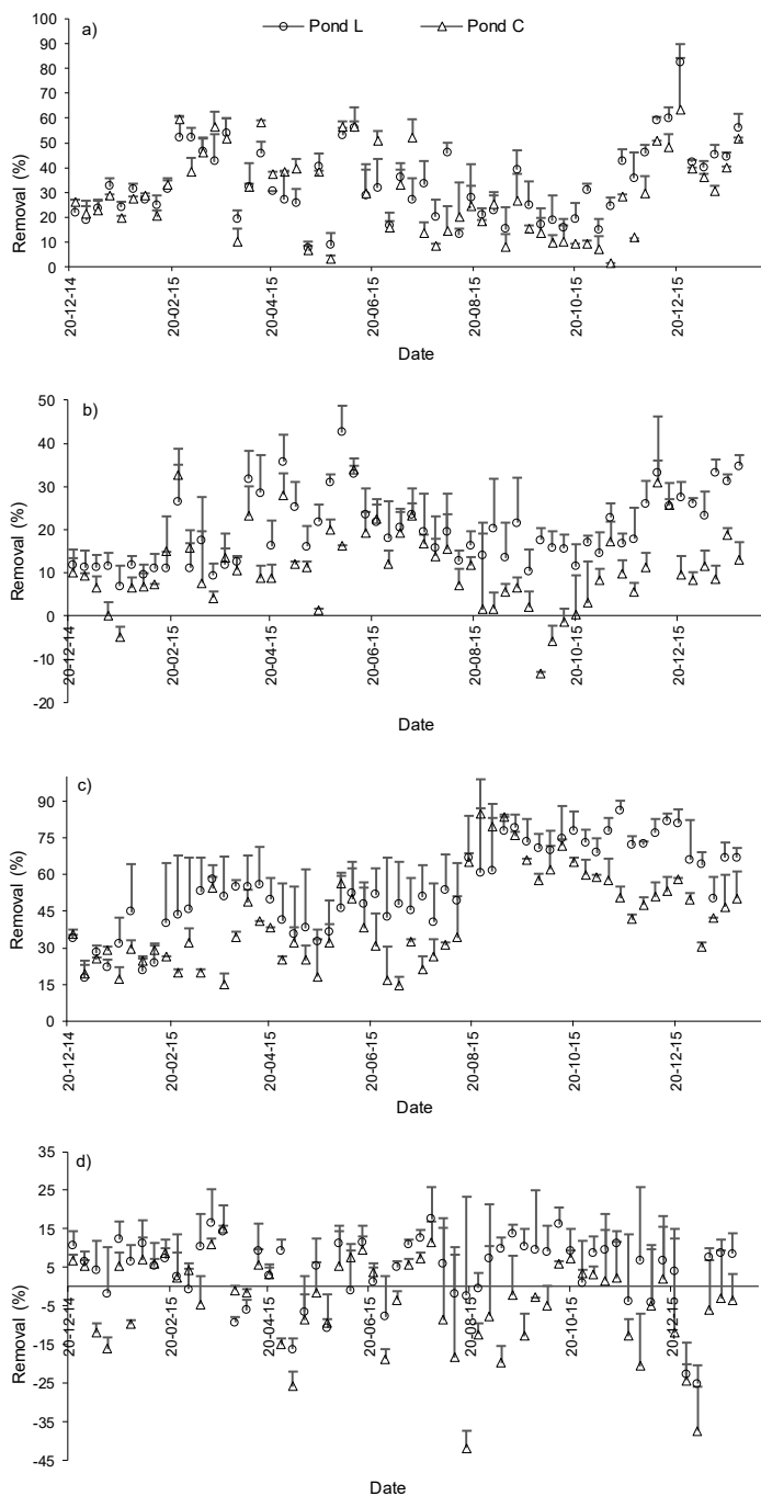
Fig. 5. Mean values of dye removal for: a) Acid Blue 113, b) Reactive Blue 198, c) Basic Red 46, and d) Direct Orange 46; L – Lemna minor L., C – control
