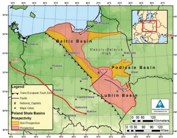
Fig. 1. The assessment of possible occurrence of the most prospective areas for shale gas deposits. (Source: US Energy Information Administration, World Shale Gas Resources: An Initial Assessment of 14 Regions Outside the United States, US Energy Information Administration (EIA) –prepared for EIA by Advanced Resources International, Inc., 2011)
