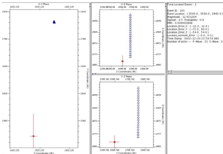
Fig. 8. Location of synthetic event in velocity model from figure 5 using downhole array
