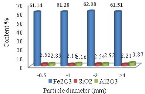
Fig. 11. Content evolution of Fe 2 O 3 , SiO 2 and Al 2 O 3 in the sample washed with water (concentrate) of Test n° 2.
