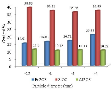
Fig. 12. Content evolution of Fe 2 O 3 , SiO 2 and Al 2 O 3 in the sample washed with water (rejected) of Test n° 1.
