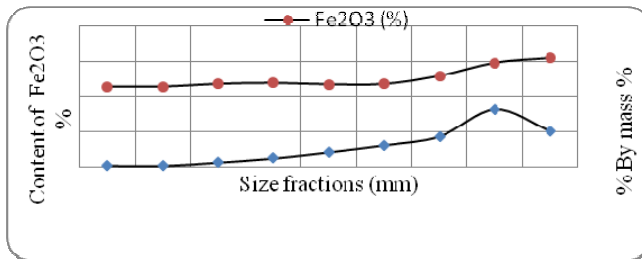
Fig. 1. Particle size analysis of Anini iron ore
