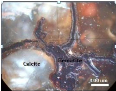
Fig. 5. Calcite associated with hematite (PL)
