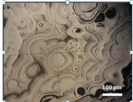
Fig. 4. Goethite of a collomorphe structure (NL)
