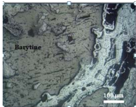
Fig. 6. Barite cracked with triangular pits (NL)
